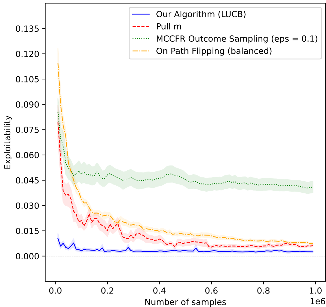
Leduc Poker, Best Algorithms, Player x
